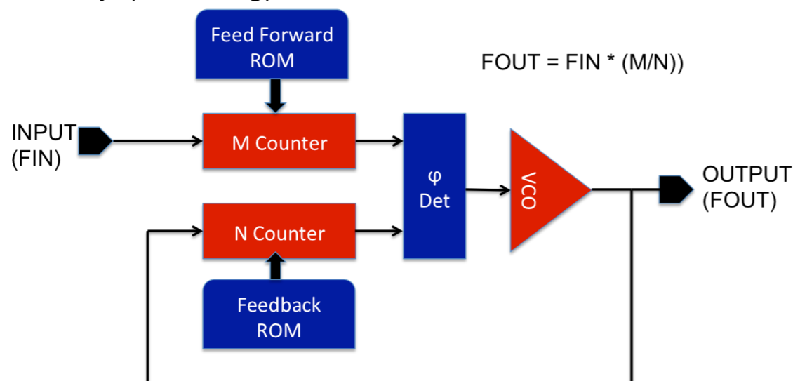
Figure 1 – PLL Based Implementation of Active EMI Management
