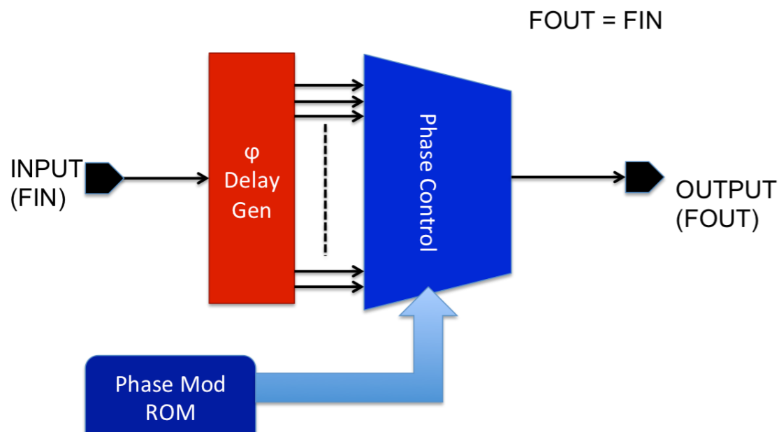
Figure 2 – SAΦIC™ Implementation of Active EMI Management
